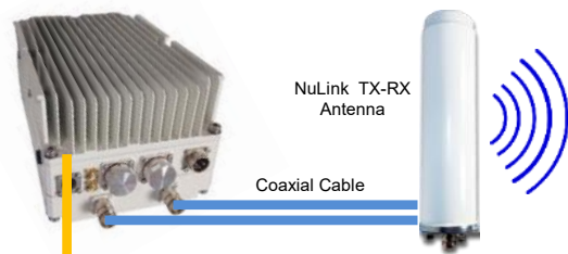
NuLink 5G Radio Head
